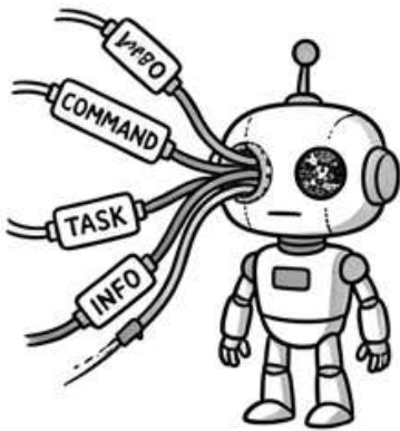
Buffer Overflow
